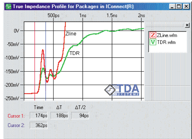
Figure 6. True impedance profile (Zline.wfm) vs. the raw TDR waveform (TDR.wfm) for a BGA package. The true impedance profile provides much more accurate information about the failure location.
